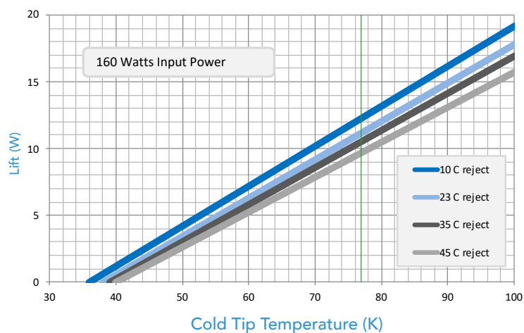
Nominal Performance at Different Reject Temperatures
